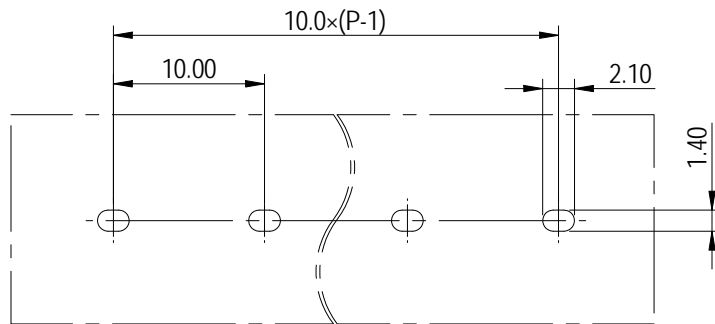
PCB LAYOUT
